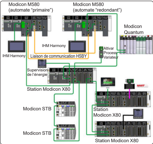
Architecture mixte RIO/DIO
